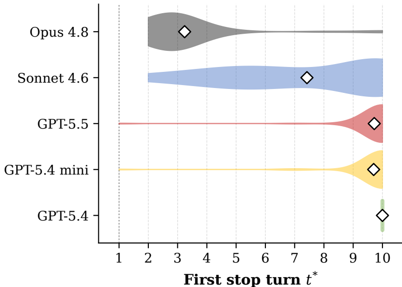
Algorithms
