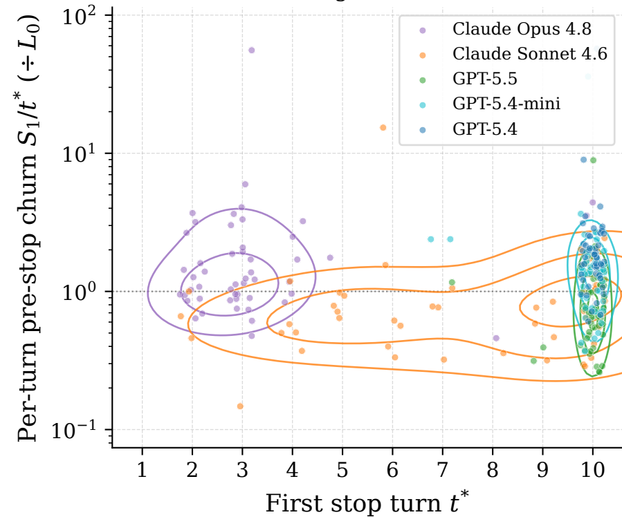
Algorithm
