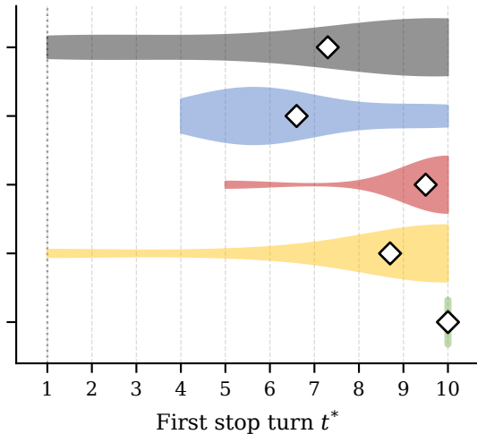
When agents stop editing an already-optimized codebase ( t^* per run; \blacklozenge = mean over all runs) Algorithms (001-050) (n=50) RealWorld (R001-R010) (n=10)
