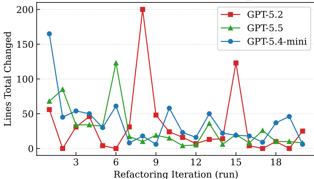
Lines Changed per Refactoring Run — BUBBLE_SORT-DASH-TEMP0.0
