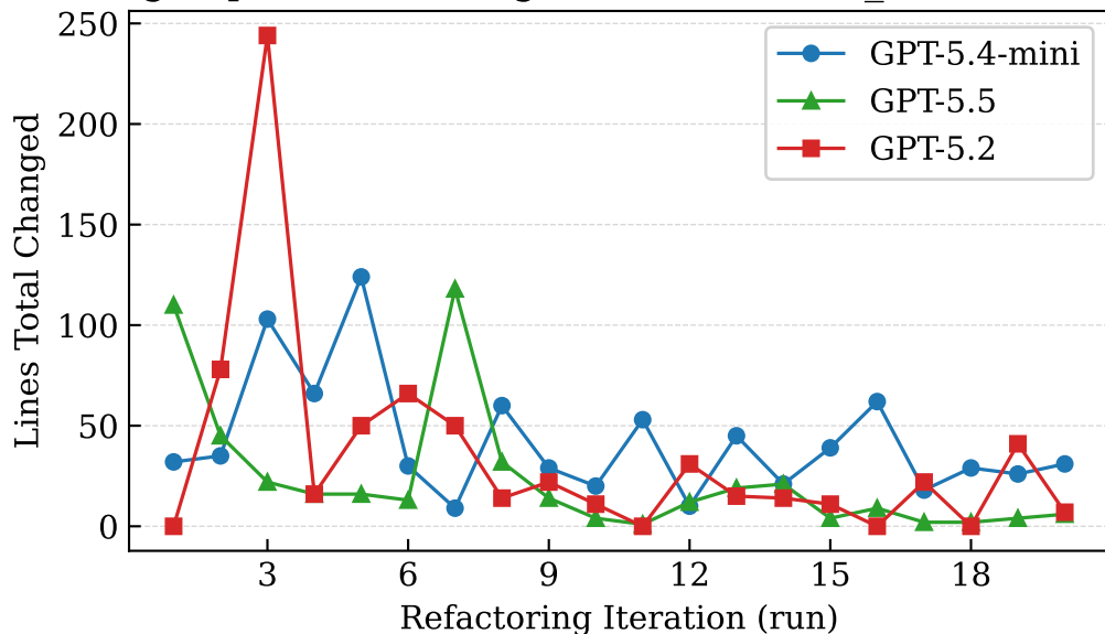
Lines Changed per Refactoring Run — BUBBLE_SORT-DASH-TEMP0.2
