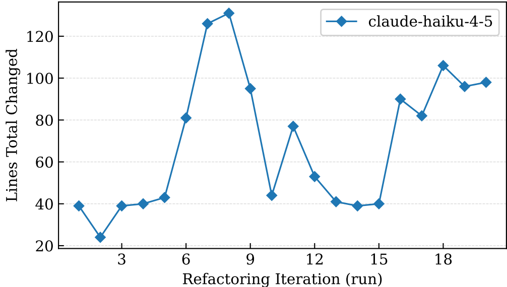
Lines Changed per Refactoring Run — BUBBLE_SORT_JAVA-CLAUDE-AGENT
