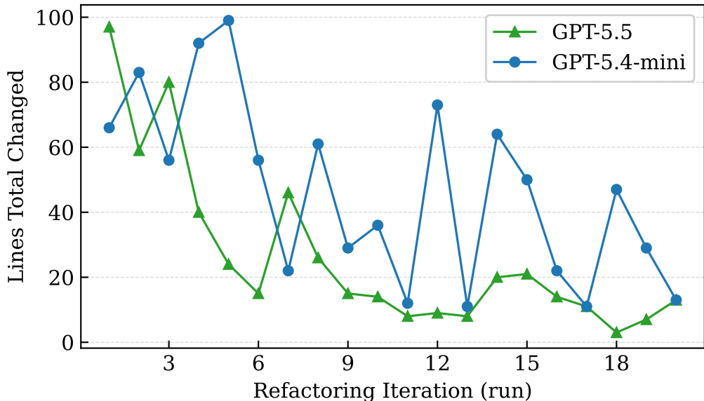
Lines Changed per Refactoring Run — EXP-APP-JAVASRIPT-TEMP0.0
