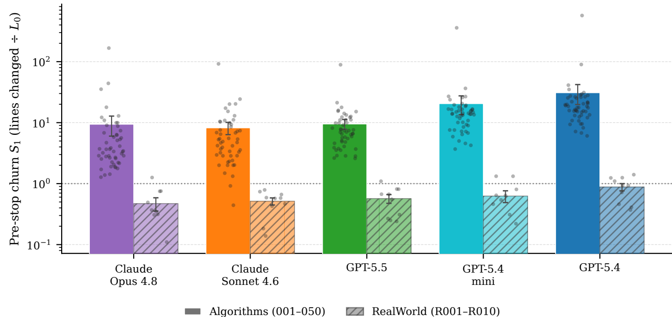
Unjustified churn before stopping (mean \pm SEM; dots = runs)
