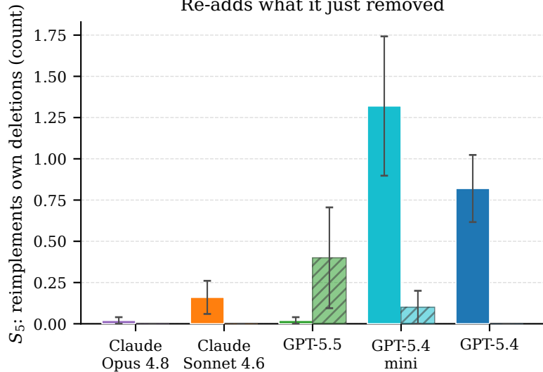
Re-adds what it just removed
