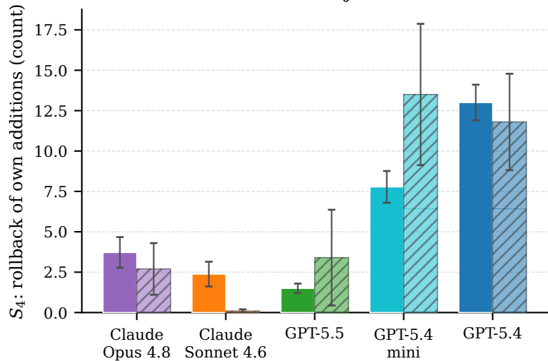
Removes what it just added
