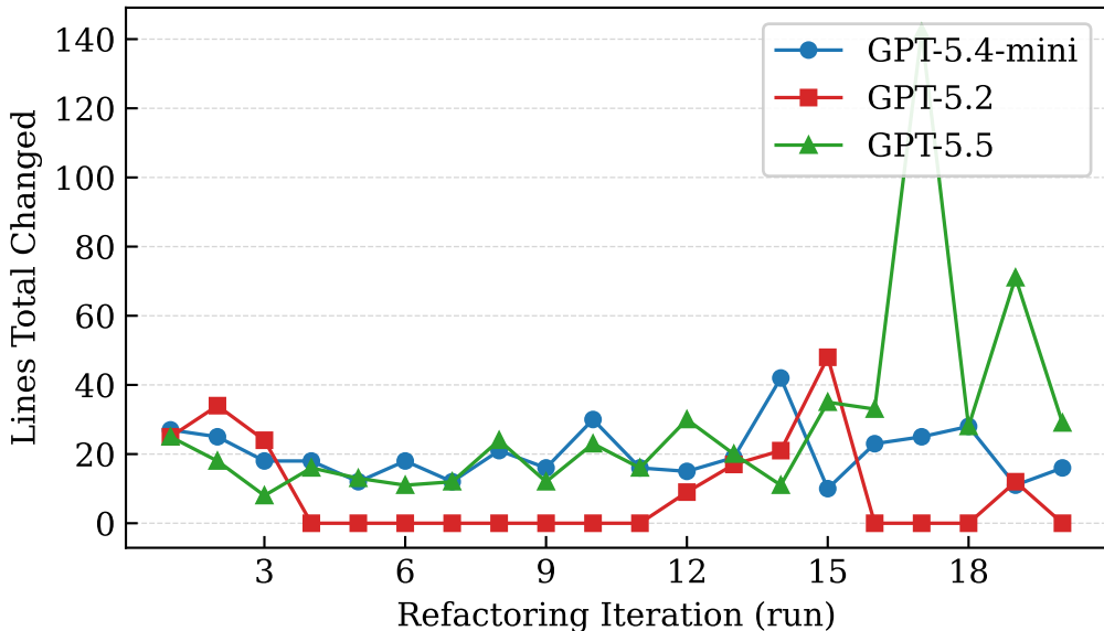
Lines Changed per Refactoring Run — TARGET
