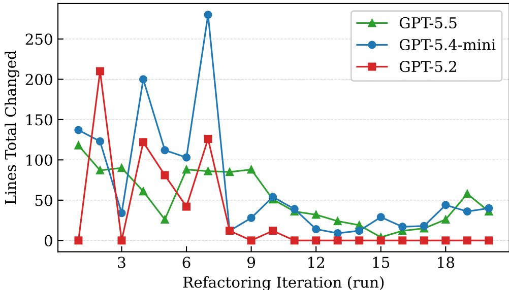
Lines Changed per Refactoring Run — TARGET2-NEW
