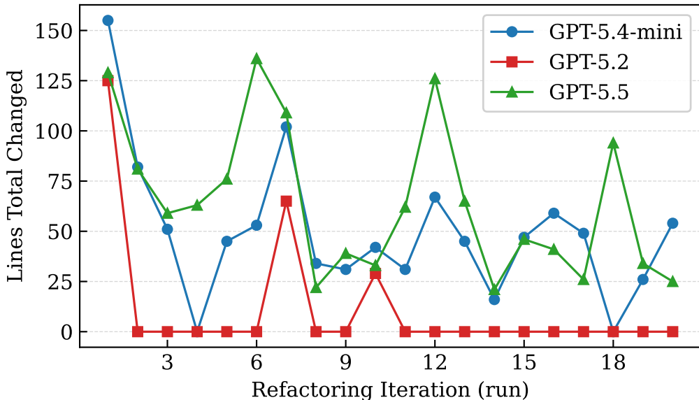
Lines Changed per Refactoring Run — TARGET2
