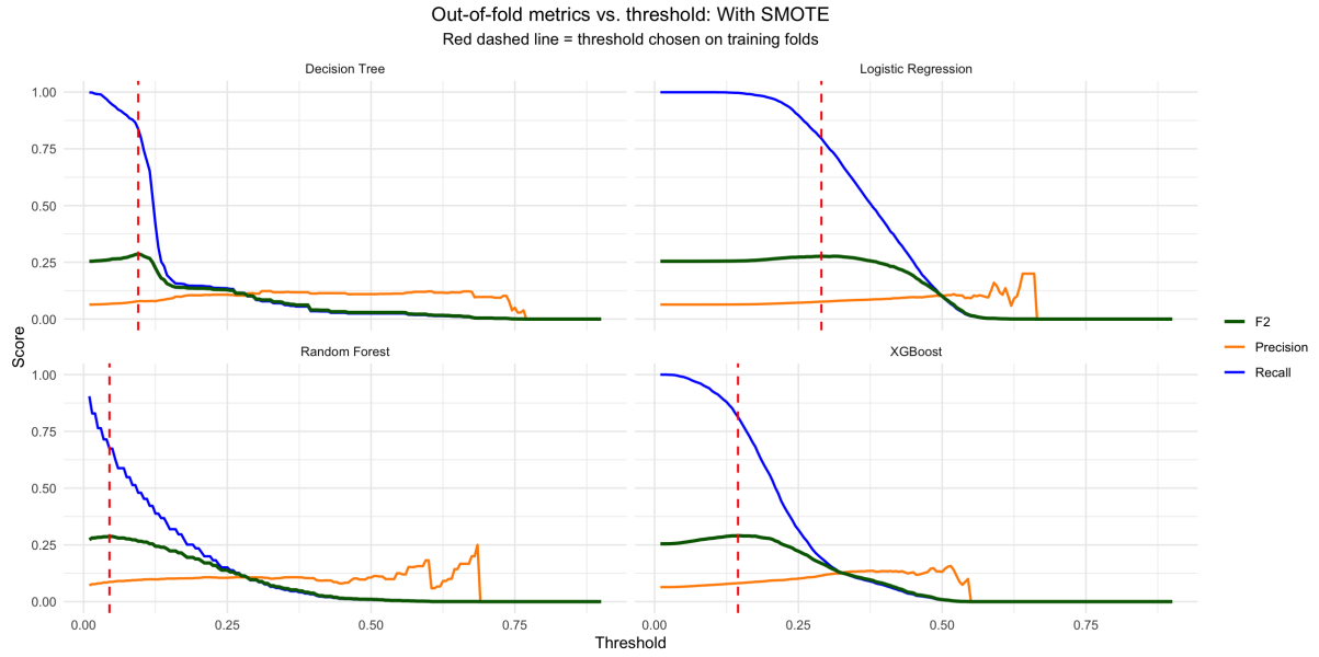
Figure 6: Out-of-fold precision, recall and F_2 versus classification threshold for each model. Red dashed lines mark the thresholds selected on the training folds.
