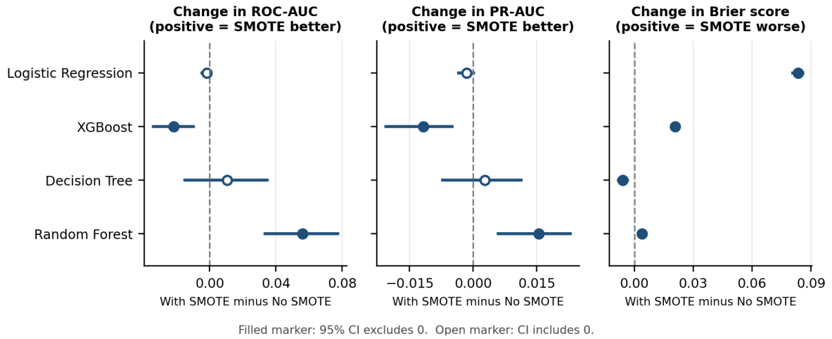
Figure 4: Effect of SMOTE (With SMOTE minus No SMOTE) on ROC-AUC, PR-AUC and Brier score, with 95% paired-bootstrap intervals.
