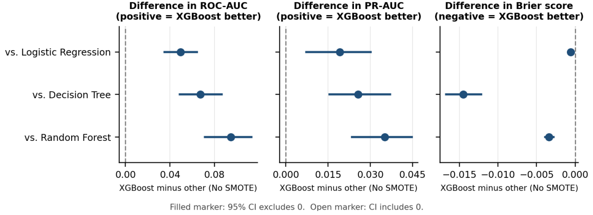
Figure 3: Paired differences between XGBoost and each other model without SMOTE, with 95% bootstrap intervals.
