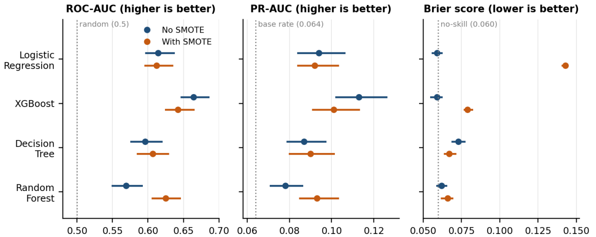
Figure 1: Test-set ROC-AUC, PR-AUC and Brier score with 95% bootstrap confidence intervals. Dotted lines are no-skill references.
