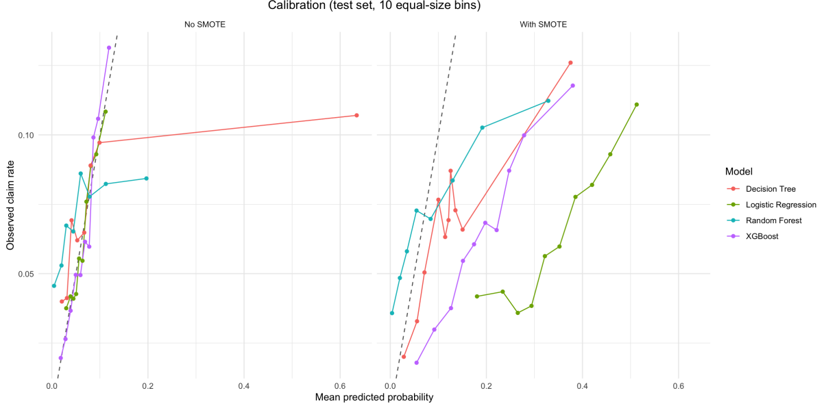
Figure 5: Calibration on the test set (ten equal-size bins of predicted probability). Points on the dashed diagonal indicate predicted probabilities that match observed claim rates. The SMOTE models generally lie below the diagonal, indicating systematic overprediction of claim probabilities, whereas the no-SMOTE models are much closer to the diagonal.
