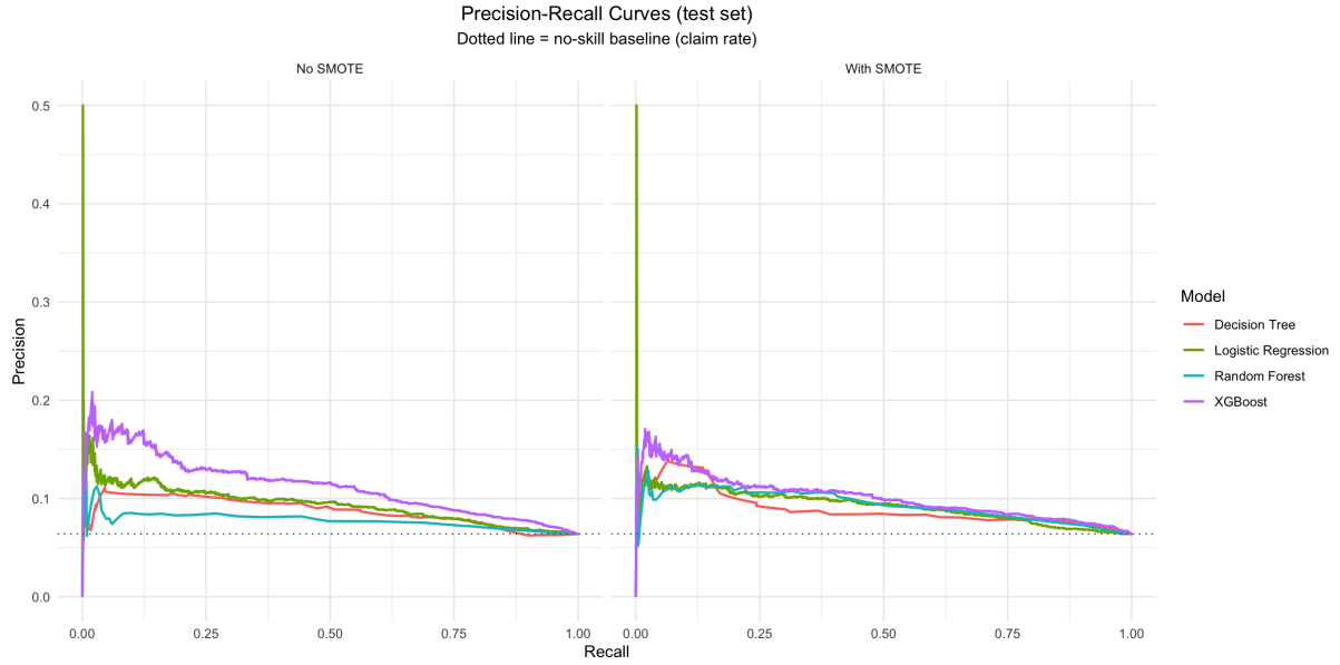
Figure 2: Precision–recall curves on the test set for each model, without SMOTE (left) and with SMOTE (right). The dotted line is the no-skill baseline (claim rate 0.064).
