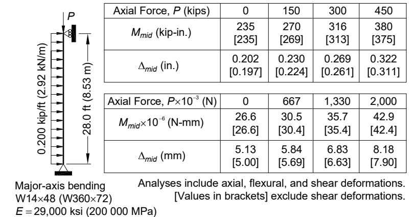
Fig. C-C2.2. Benchmark problem Case 1.
