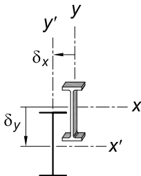
(b) Member twist not considered
