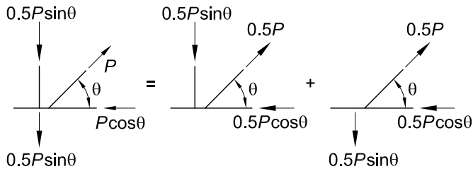
Fig. C-K1.2. Checking of K-connection with imbalanced branch member loads.
