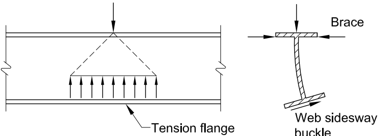
Fig. C-J10.2. Web sidesway buckling.
