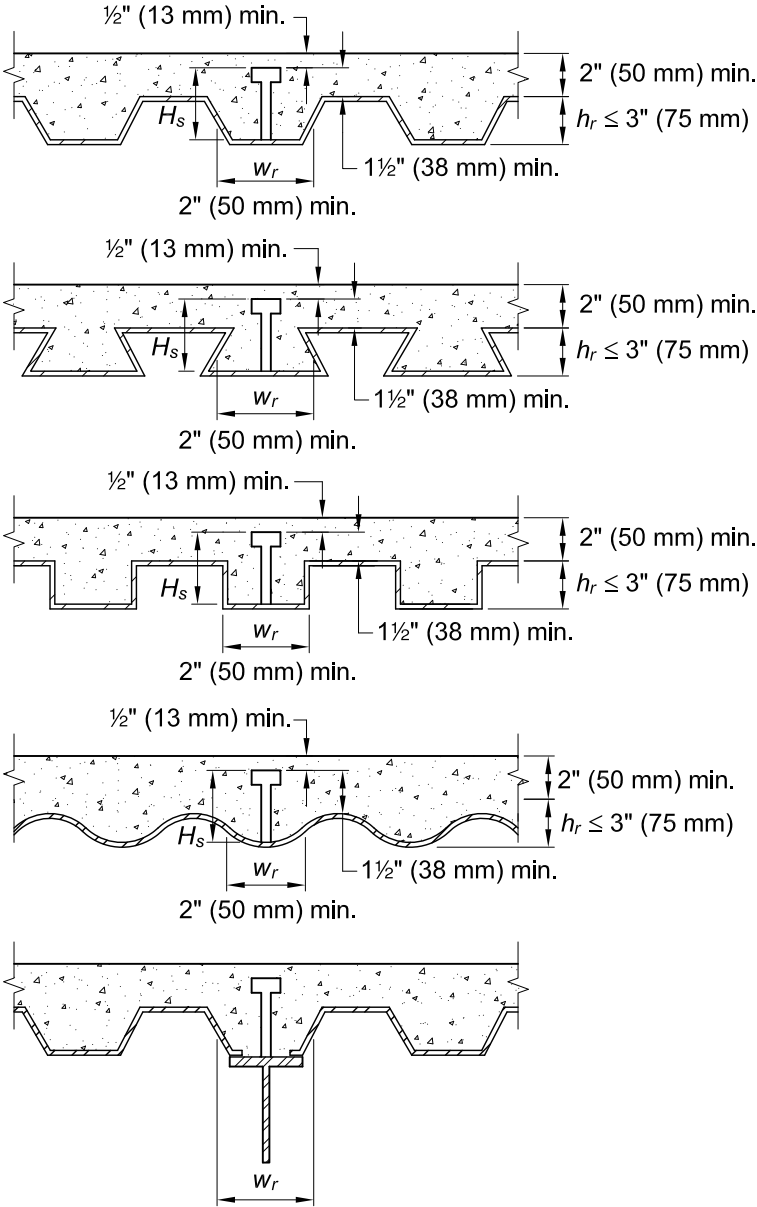
Fig. C-I3.6. Steel deck limits.
