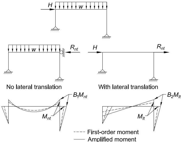
Fig. C-A-8.1. Moment amplification.
