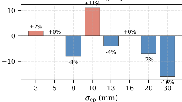
Belief PPO advantage by noise level
