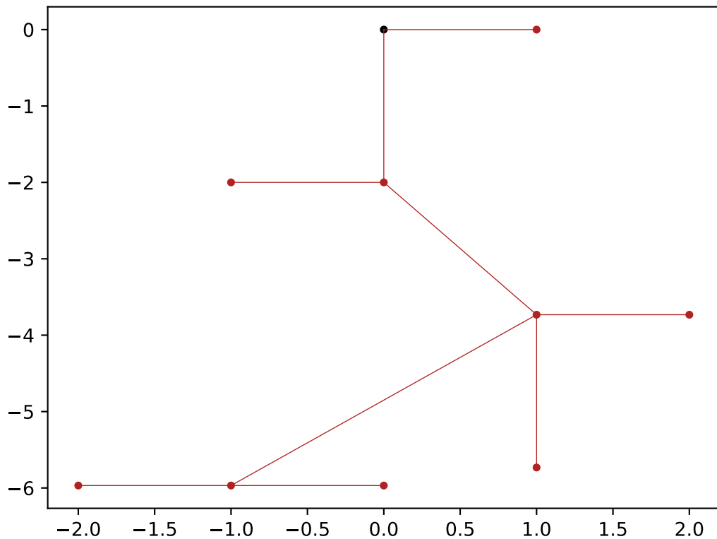
tree2.swc
