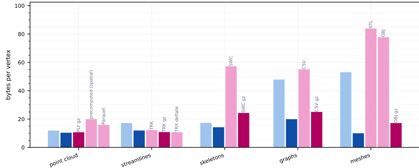
Storage per vertex ( N \approx 10,000,000 )
