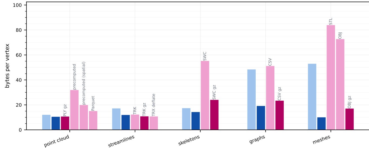
Storage per vertex (N \approx 1,000,000)
