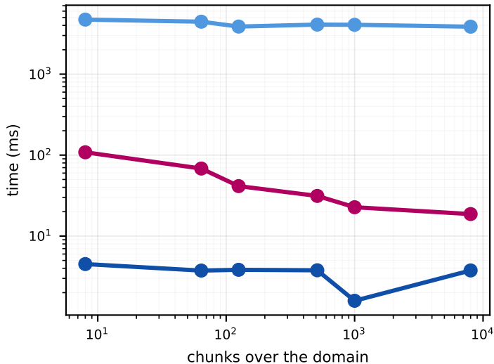
Read one large object vs chunk count ( N = 1\text{M} vertices)
