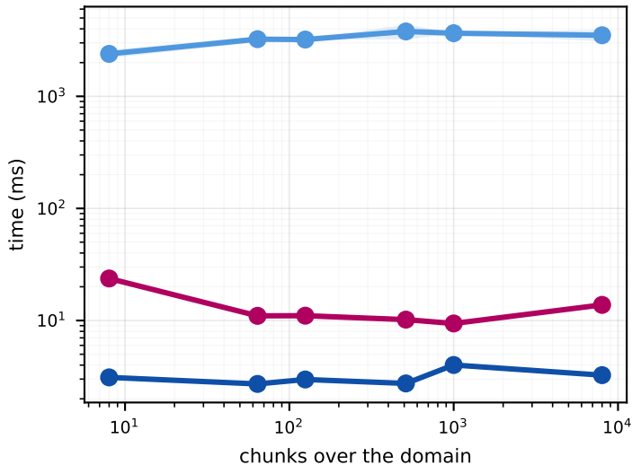
Read one object vs chunk count (N = 1.0M vertices)
