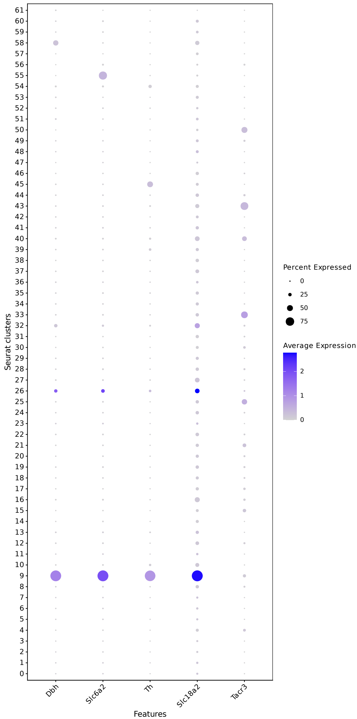
Marker expression by cluster
