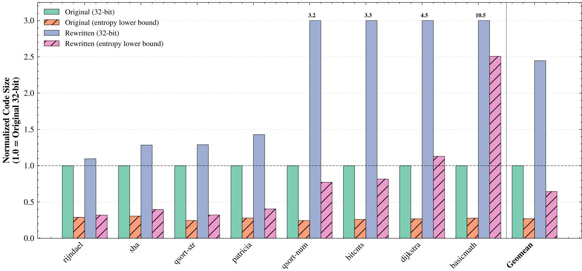
Entropy Lower Bound — MIBENCH
