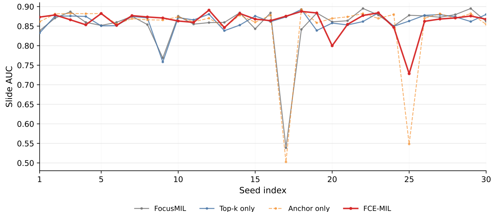
Camelyon17 ResNet18 ablation across 30 seeds
