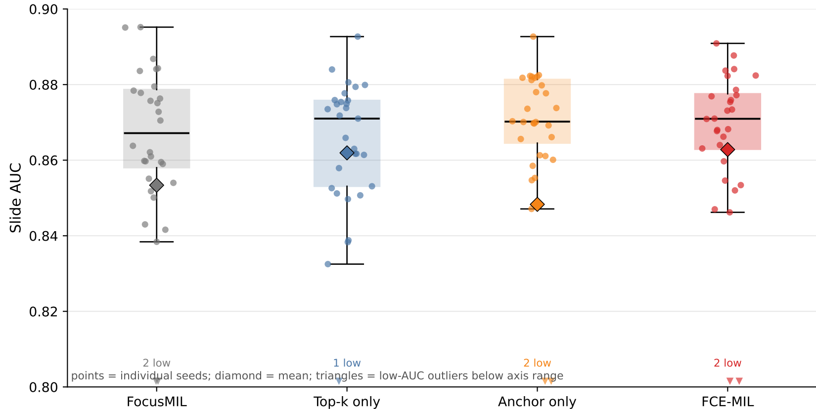
Camelyon17 ResNet18 ablation across 30 seeds
