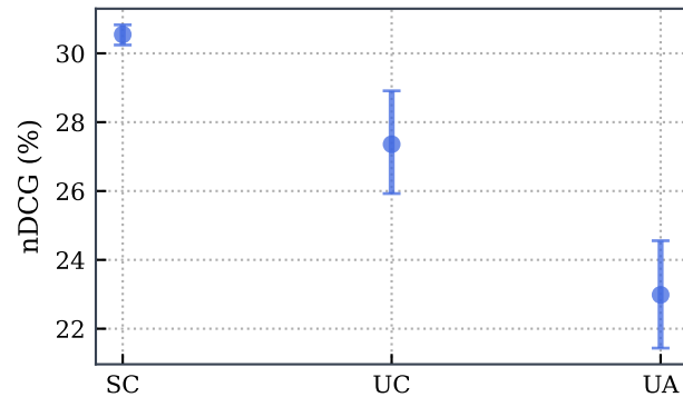
(b) V→T nDCG
