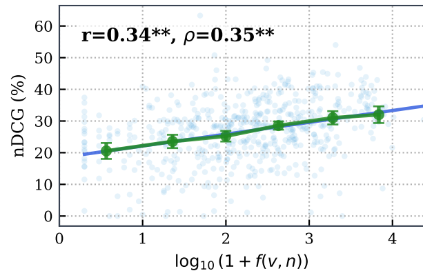
(f) V→T nDCG
