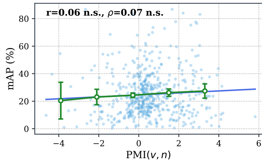
(c) T→V mAP
