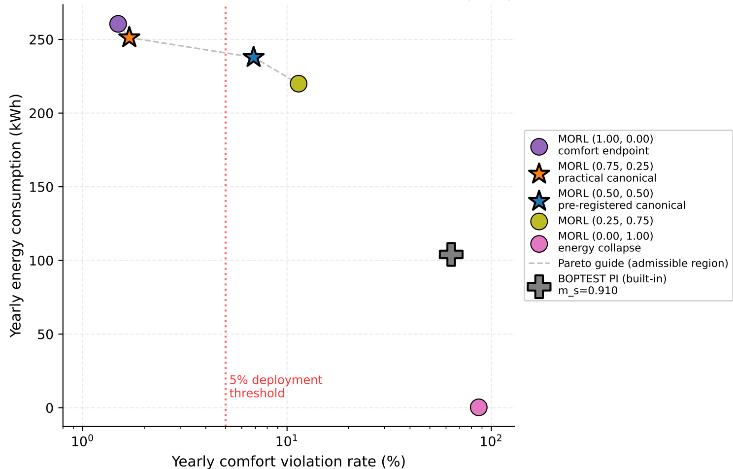
Block 2: MORL Pareto front vs BOPTEST PI baseline (yearly)
