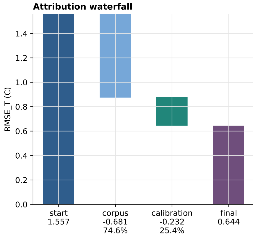
Figure 3. Matched-corpus decomposition of predictive-fidelity gain
