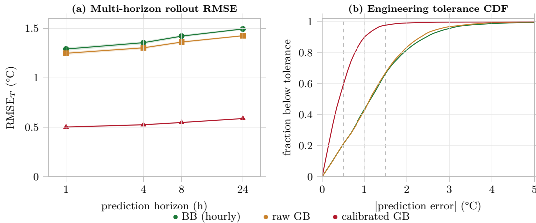
FIGURE 3. Multi-horizon predictive validity, residual spread and engineering error CDFs from BOPTTEST rollouts. The calibrated grey-box twin is the better predictor at every horizon; the coarse black-box surrogate degrades beyond a few hours yet remains the usable training environment.
