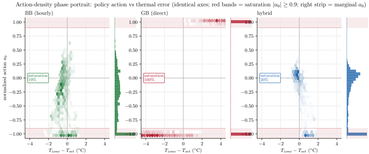
Figure S8: Action-density phase portrait of the three thermostatic controllers on the live BOPTEST typical_heat_window: empirical hexbin density of the normalized supply-temperature action a_0 (one hue per backend) against the thermal error T_{\text{zone}} - T_{\text{set}} , on identical axes, with the marginal a_0 distribution in the right strip of each panel and the measured saturation share ( |a_0| \geq 0.9 ). The red bands mark the actuator-saturation region. Direct GB collapses onto a_0 = -1 (100% saturation, a bang-bang law) whereas the usable hourly BB and the hybrid modulate ( \approx 19 –20%).
