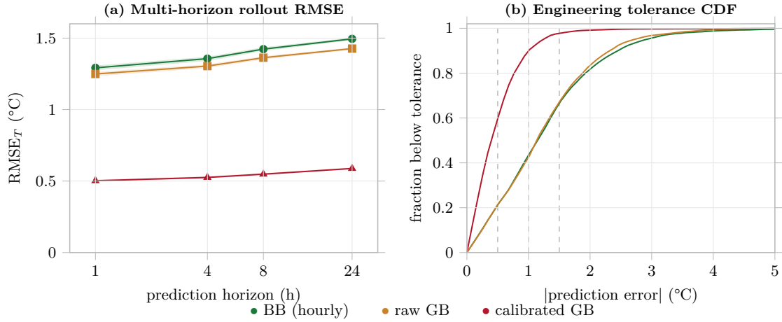
Figure 3: Multi-horizon predictive validity, residual spread and engineering error CDFs from BOPTEST rollouts. The calibrated grey-box twin is the better predictor at every horizon; the coarse black-box surrogate degrades beyond a few hours yet remains the usable training environment.
