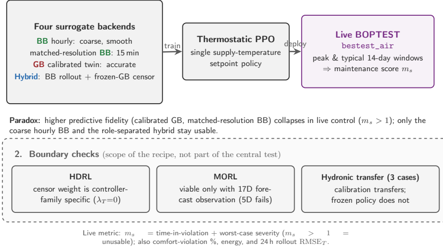
Figure 1: Study overview. Top, primary paradox test: four surrogate backends (coarse hourly BB, matched-resolution BB, calibrated GB, and the role-separated hybrid) each train a thermostatic PPO controller scored live on BOPTEST bestest_air ; the higher-fidelity backends collapse ( m_s > 1 ) while the coarse BB and the hybrid stay usable. Bottom, boundary checks (dashed box): hierarchical DRL, multi-objective RL and a three-case hydronic transfer study map the scope of the recipe and are not part of the central test.
