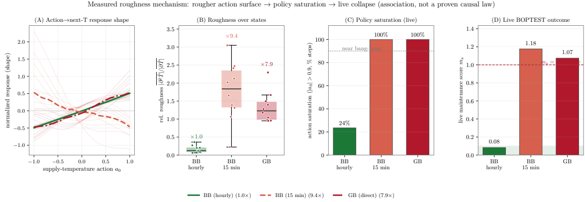
FIGURE 7. Measured roughness mechanism. The collapsing single-model backends expose rougher action–response surfaces, produce near bang-bang saturation and fail on the live emulator; the pattern is mechanistically consistent with the fidelity–utility paradox but does not by itself prove full loss-landscape causality.
