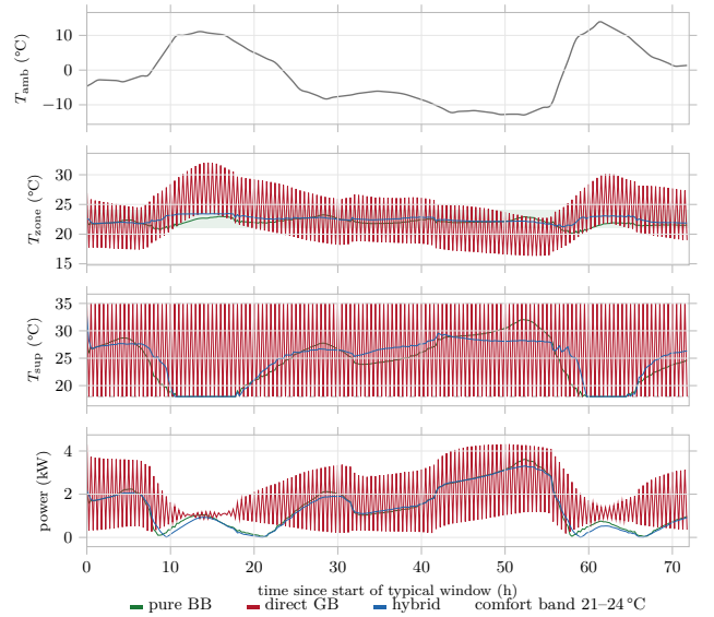
FIGURE 8. Live closed-loop behavior on the typical window: zone temperature against the comfort band, with ambient disturbance and HVAC power, for the pure-BB, direct-GB and hybrid controllers. Direct GB saturates the actuator and leaves the band; the coarse BB and the hybrid track it.
