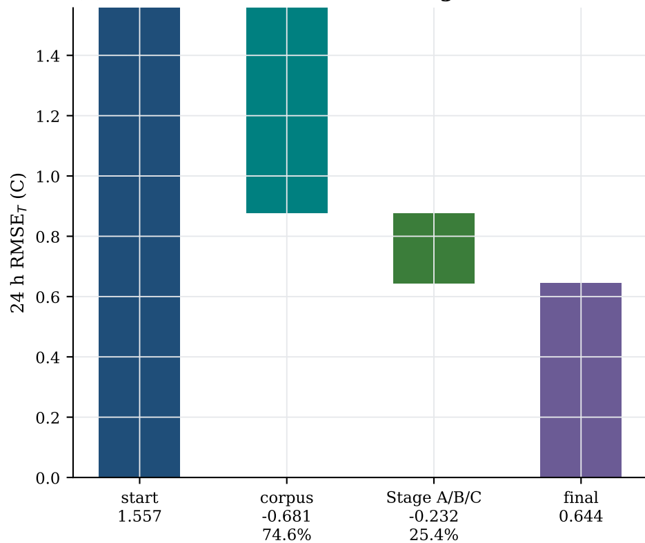
(b) Attribution of the v3-to-v3.5 gain
