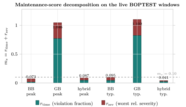
FIGURE 6. Live BOPTTEST maintenance-score decomposition. Direct GB fails through sustained out-of-band time; pure BB and the hybrid keep both duration and severity small.
