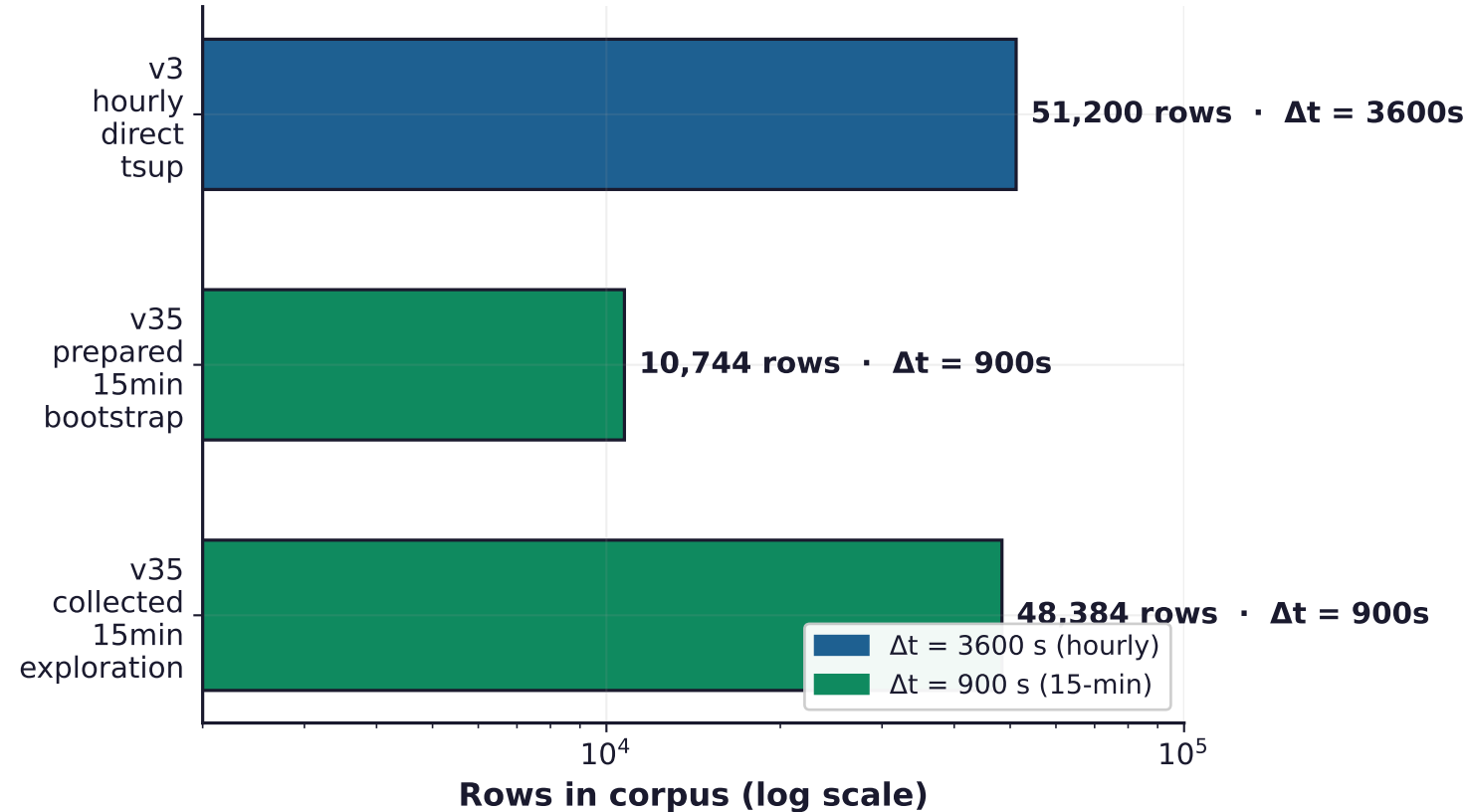
(a) Three training corpora
