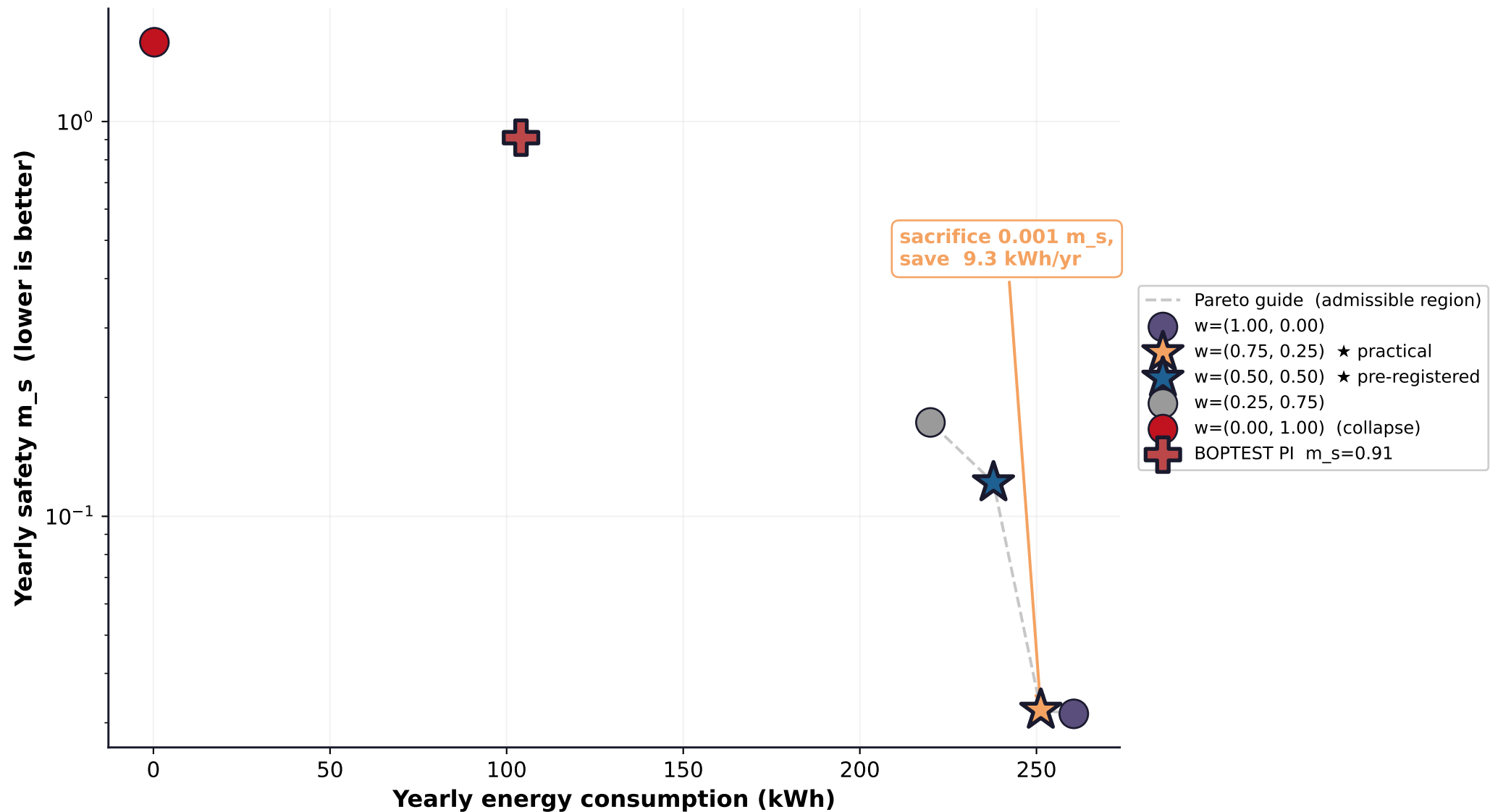
Q2.4 MORL Pareto front on (energy, m_s) axes + BOPTEST PI reference
