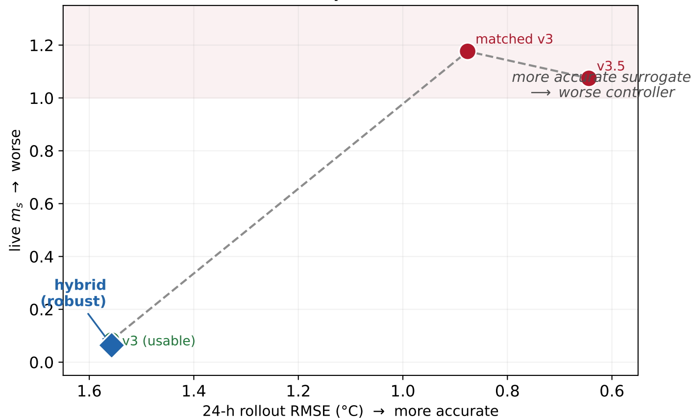
The paradox
