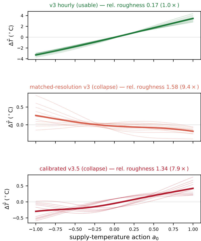
(A) Measured action \rightarrow next-temperature response over a grid of states
