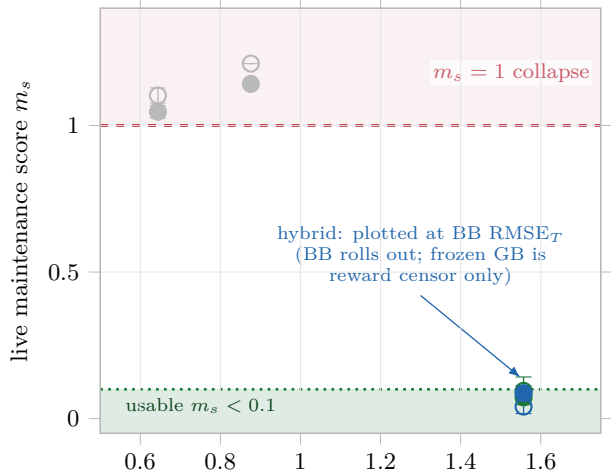
(A) Single-model paradox: more accurate \rightarrow worse live m_s (B) Role-separated hybrid recovers usable control
