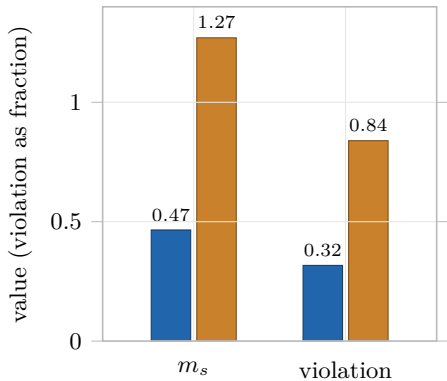
Peak KPIs: warm-start is worse
