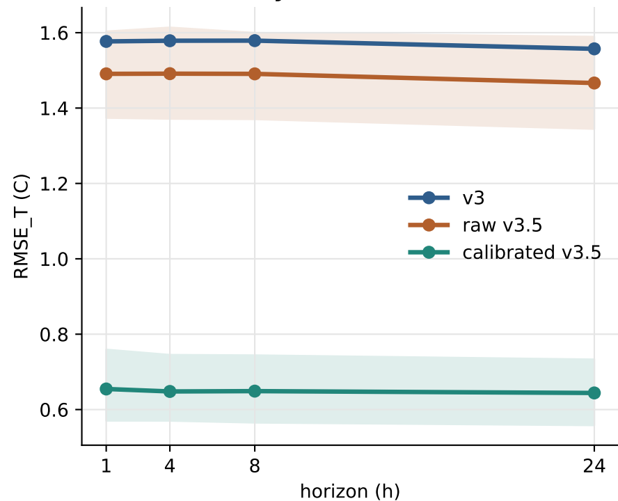
Rollout RMSE by horizon
