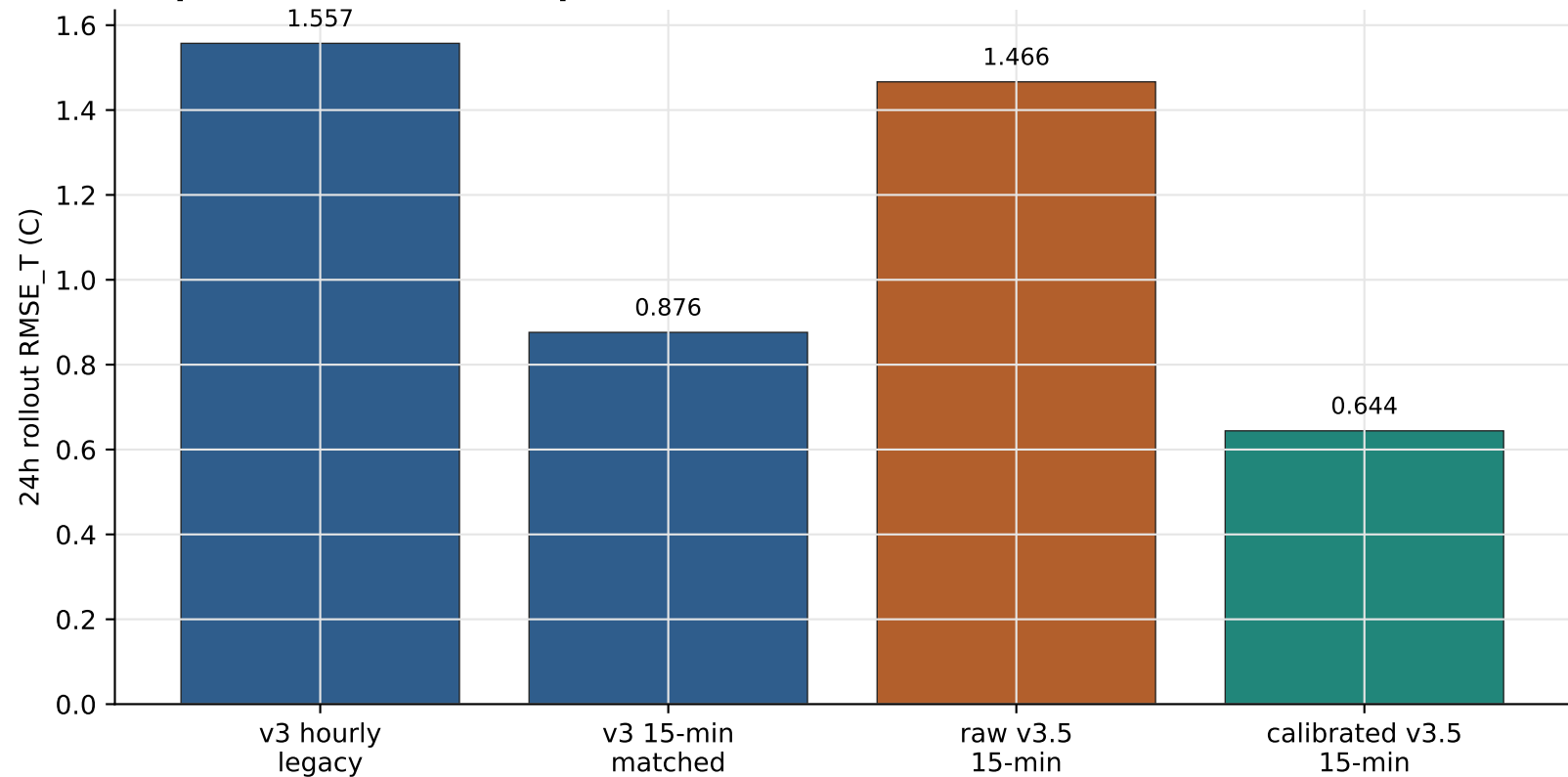
Corpus-controlled decomposition of 24h rollout RMSE
