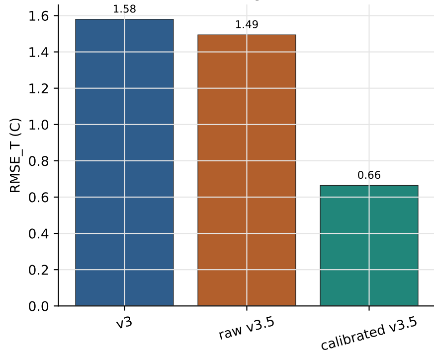
Recursive 15-min temperature error
