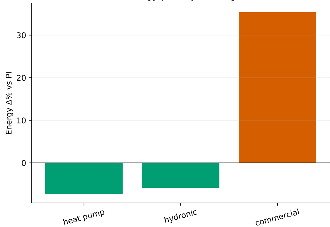
Energy penalty / saving
