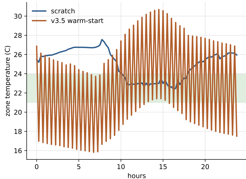
Peak-heat live trace after fine-tune
