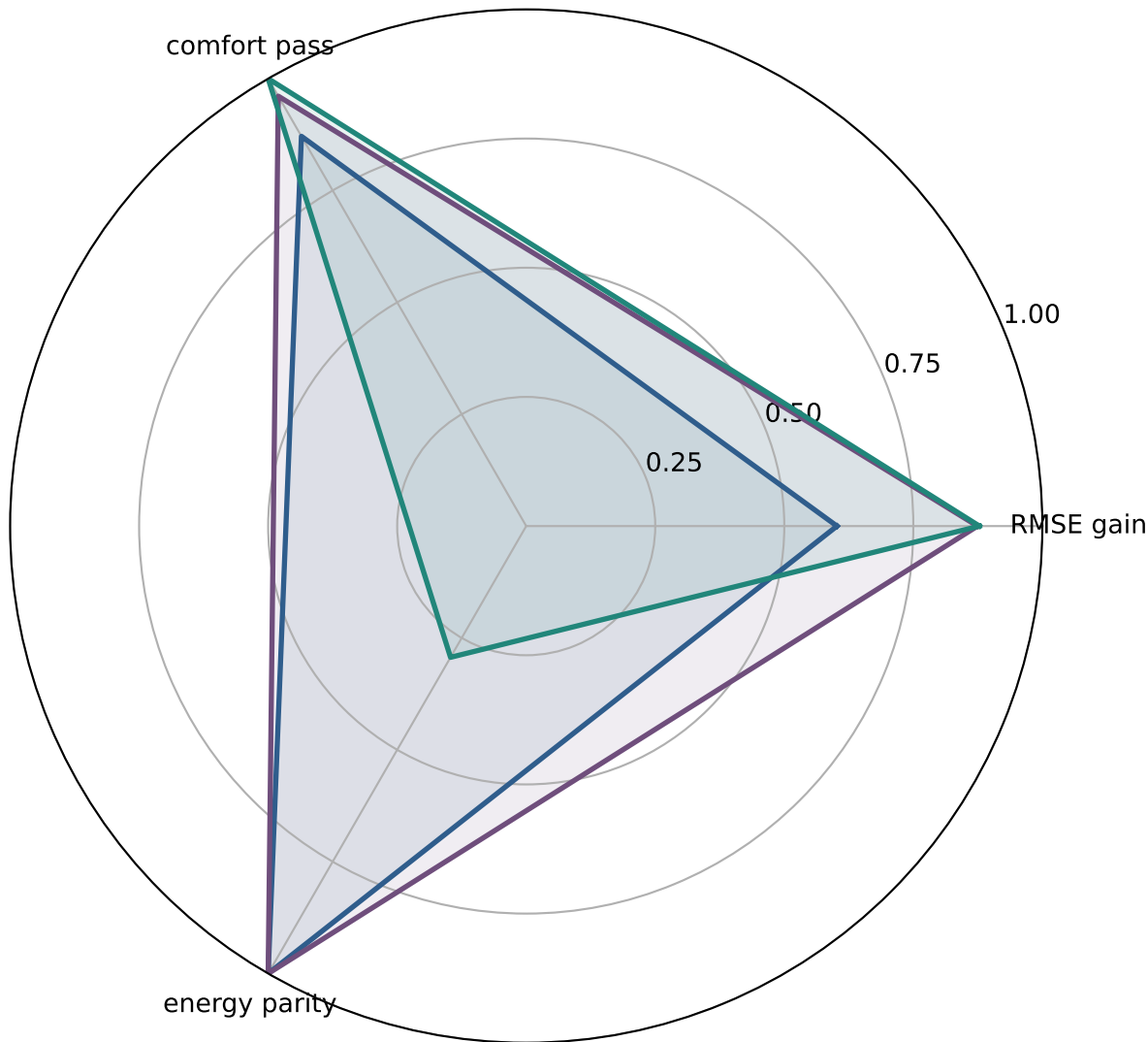
Block 3 transfer profile radar: surrogate gain vs controller deployability heat pump hydraulic commercial
