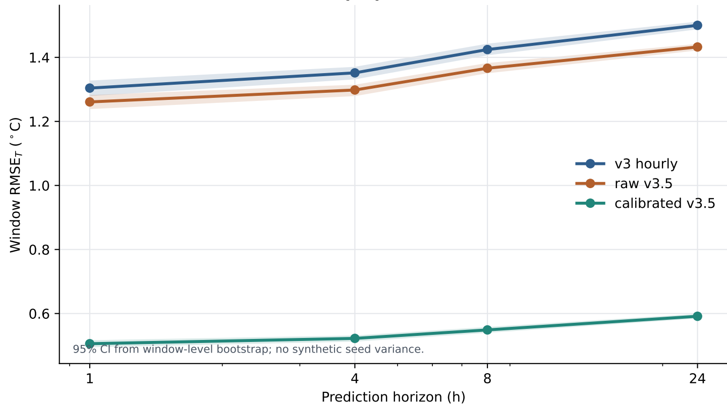
Multi-horizon rollout RMSE from prepared BOPTEST windows
