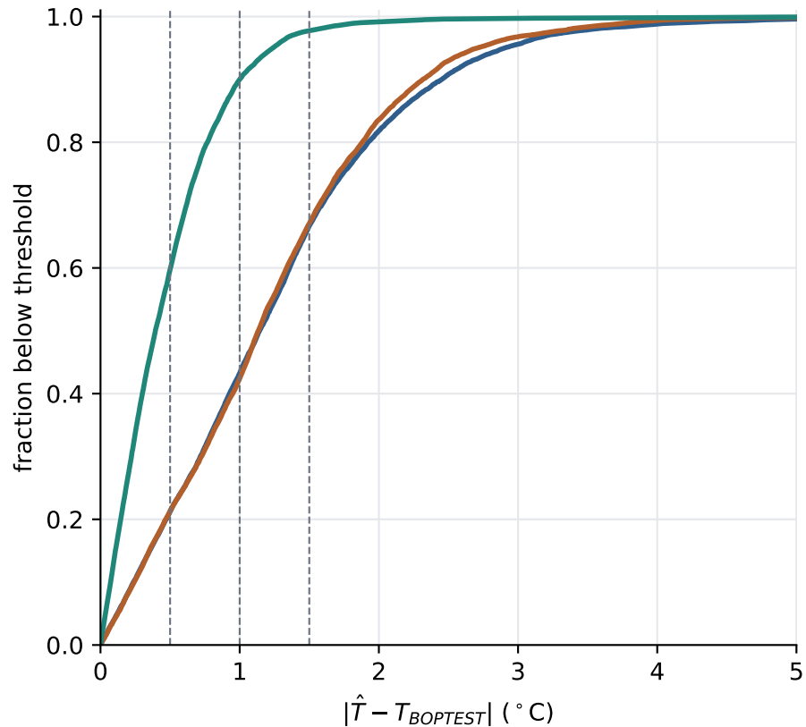
Absolute-error CDF
