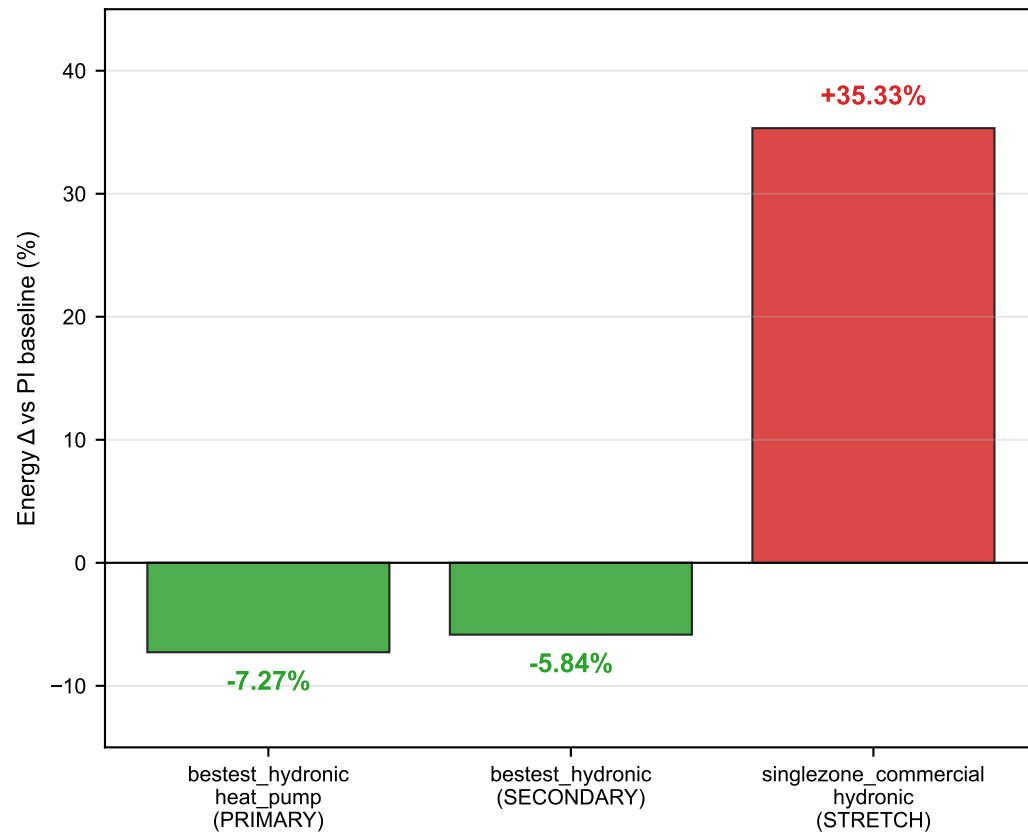
Energy delta — saves on residential, penalty on commercial
