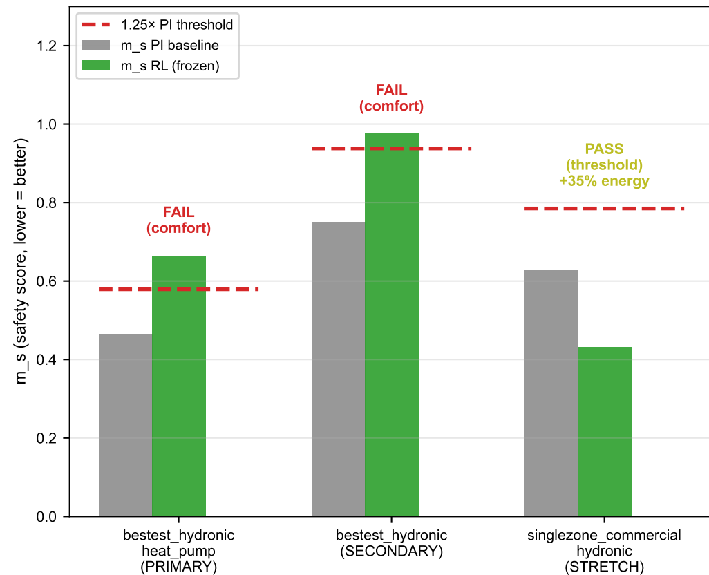
Frozen-controller vs pre-registered 1.25× PI threshold
