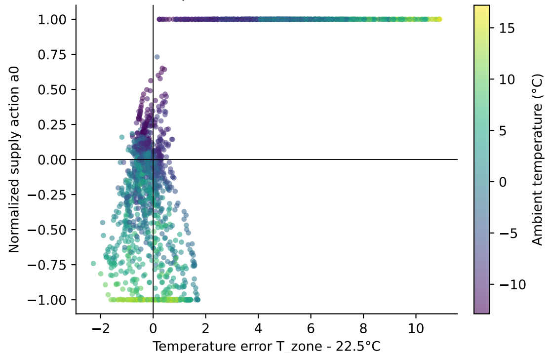
(b) Phase portrait: action vs thermal error
